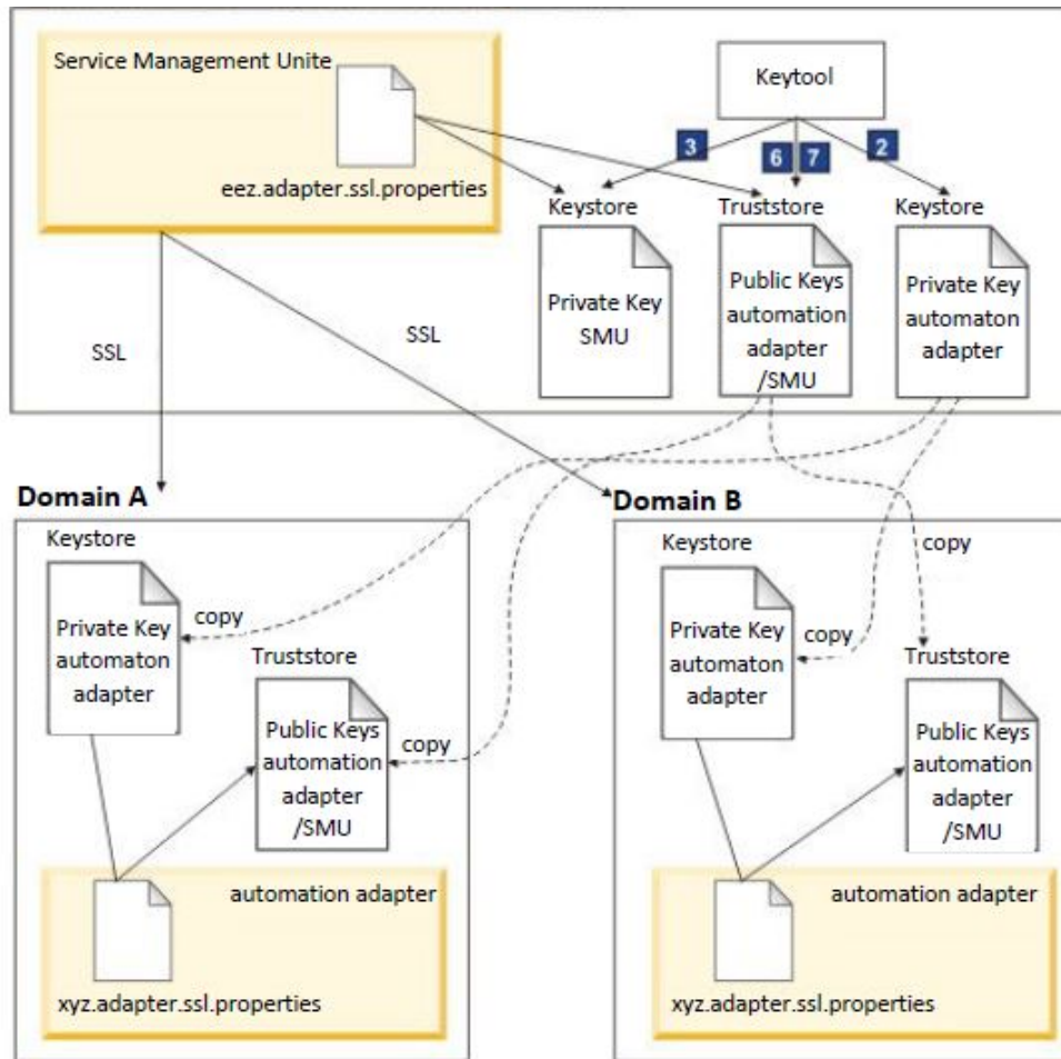
Figure 2. Keystore and truststore generation using SSL
