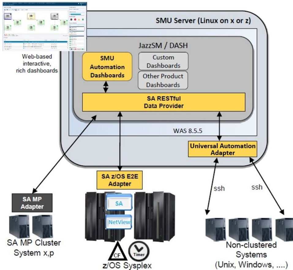
Figure 1. IBM Service Management Unite Automation architecture
